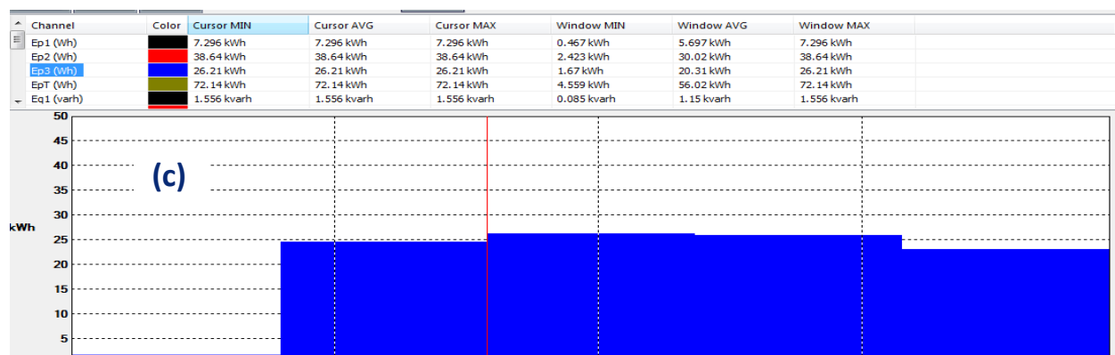
Figure 4.5 Energy Generated by 200 KVA DG Set on trial – (a) Phase-1, (b) Phase-2, and (c) Phase-3.
