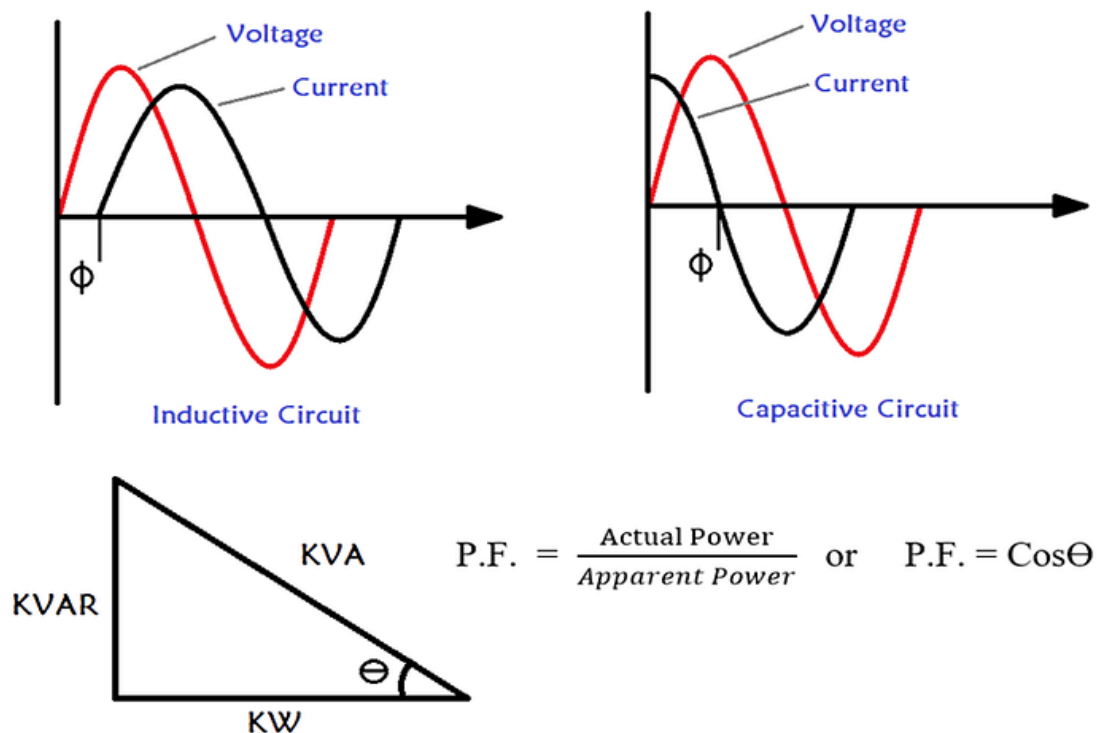
Figure 4.13 Power Factor Waveform
