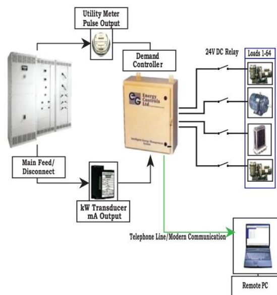
Figure 4.15 Direct demand monitoring
